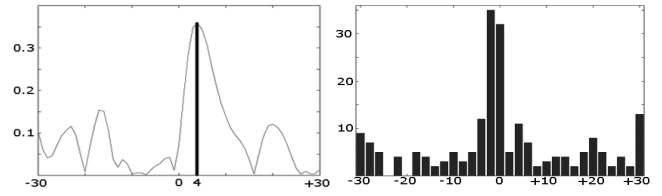
Fig. 3. Example of L_{max}(X) and its distribution on 208 synchronised sequences
